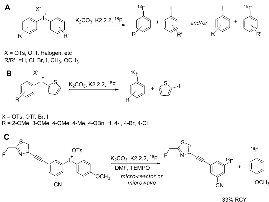
Figure 8. ^{18}\text{F} -Aromatic nucleophilic substitution on diaryliodonium salts. (A) ^{18}\text{F} -Labeling on dihomoiaryliodonium. 54 (B) ^{18}\text{F} -Labeling of aryl(2-thienyl)iodonium salts. (C) ^{18}\text{F} -Labeling on 3-cyano-5-((2-(fluoromethyl)thiazol-4-yl)ethynyl)phenyl(4-methoxyphenyl) iodonium salt. 57
