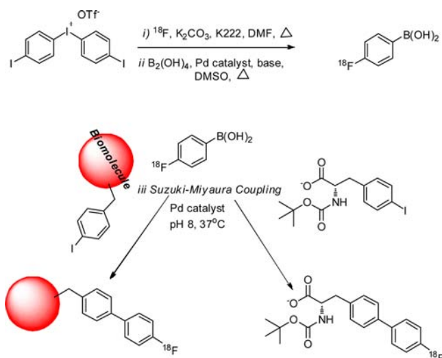
Figure 17. Suzuki–Miyaura coupling via 4- ^{18}\text{F} -fluorophenylboronic acid prosthetic group. 100
